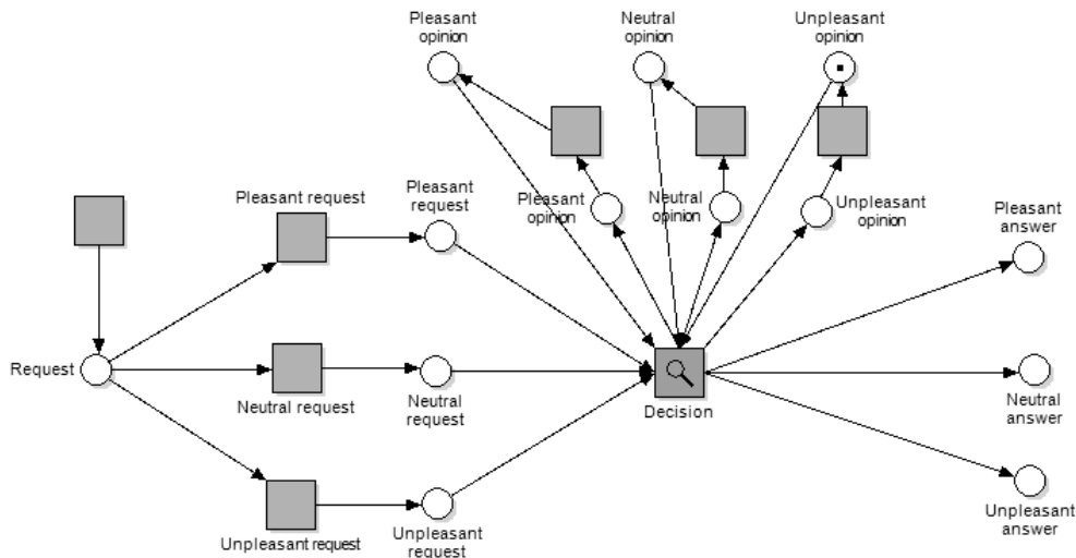
Figure 11: Request-answer process
