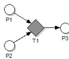
Figure 8: XOR-join transition
